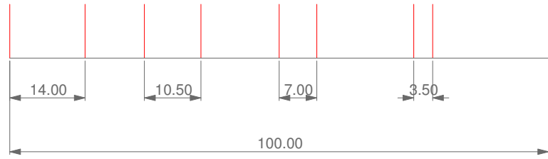
Gauge for the width of the gores of the Gorewood One Sheet Canoe designed by flo-mo
